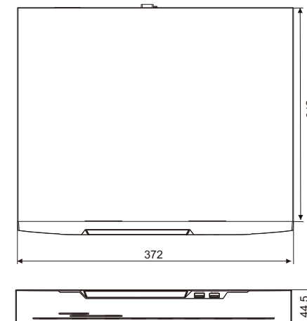
Figure 2-1 Dimensions (Unit:mm)
